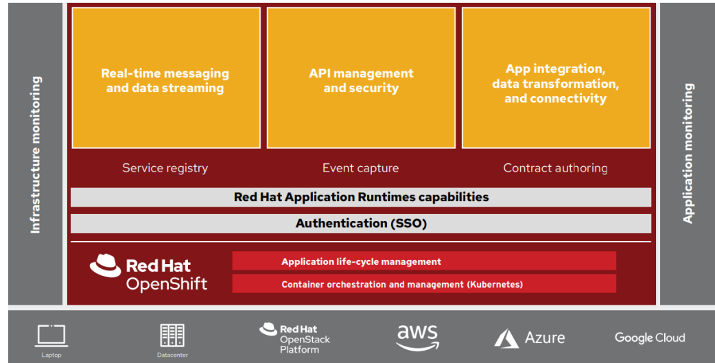
Figure 1. Red Hat Integration capabilities
